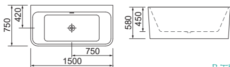
BG-1016C 1500 x 750 x 580mm
